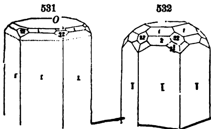
Haddam, Ct.
